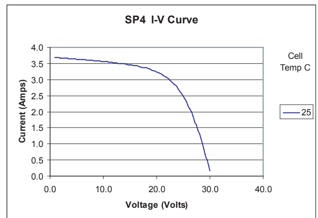
The I/V graphs above show the typical performance of the solar module at STC
